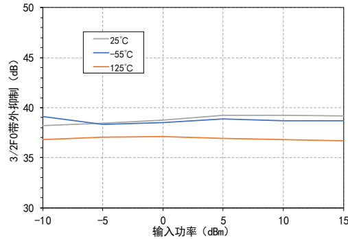
3/2F0带外抑制VS输入功率@Vt=12V
