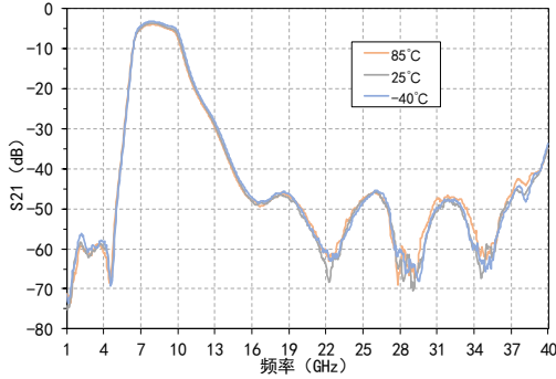
S21 VS 频率@Vt=15V
