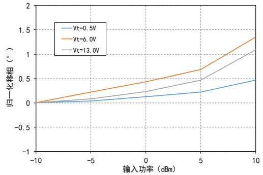
归一化移相VS Pin@10GHz
